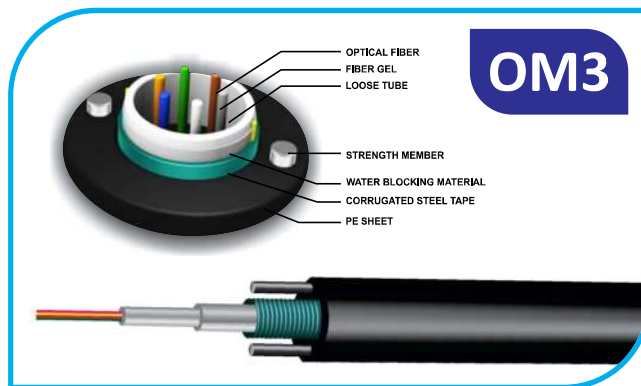
6,12,24 CORE MULTI MODE INDOOR/OUTDOOR ARMOURED FIBER OPTIC CABLE OM3
