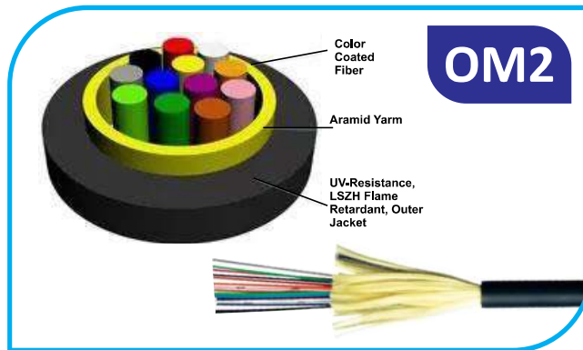
6,12,24 CORE MULTI MODE INDOOR/OUTDOOR FIBER OPTIC CABLE OM2
