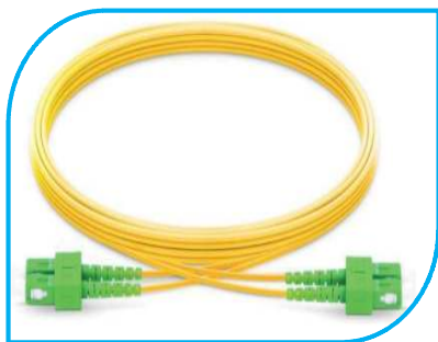
(1, 2, 3, 5, 10, 15, 20, 25, 30) M SINGLE MODE SC-SC/APC DUPLEX FIBER OPTIC PATCH CORD LSZH
