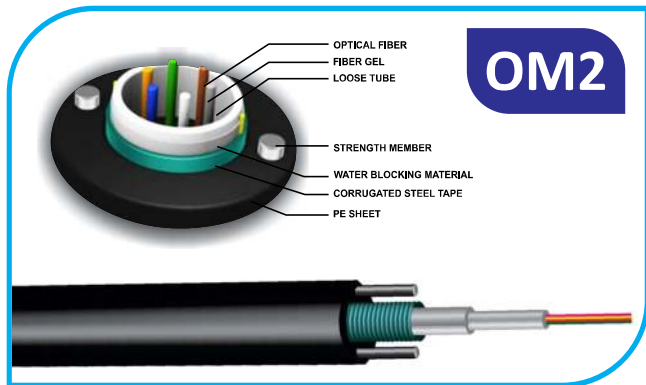
6,12,24 CORE MULTI MODE INDOOR/ OUTDOOR ARMOURED FIBER OPTIC CABLE OM2
